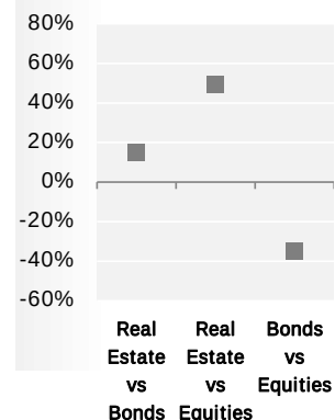
Correlation (3 yr. rolling)
